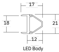
SLT 35409 Profile Dimension
