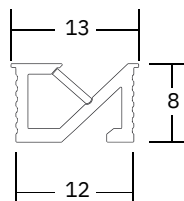
SLT 36411 Profile Dimension
