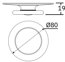
SLT 32311 & SLT 32411 Profile Dimension
