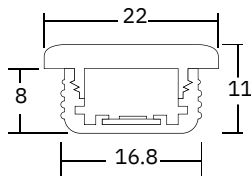
SLT 32306 & SLT 32406 Profile Dimension
