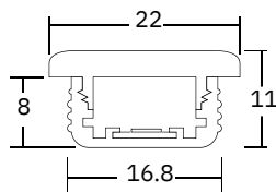
SLT 32405 & SLT 32305 Profile Dimension
