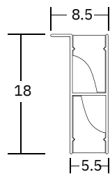
SLT 33400 Profile Dimension
