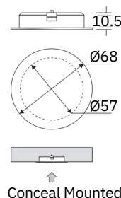
Conceal Mounted
