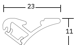
SLT 36406 Profile Dimension
