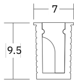
SLT 36408 Profile Dimension
