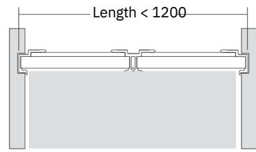
Backlit Panel Extension Top View
