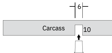
Top Mounted
