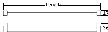
SLT 34402 Dimension
